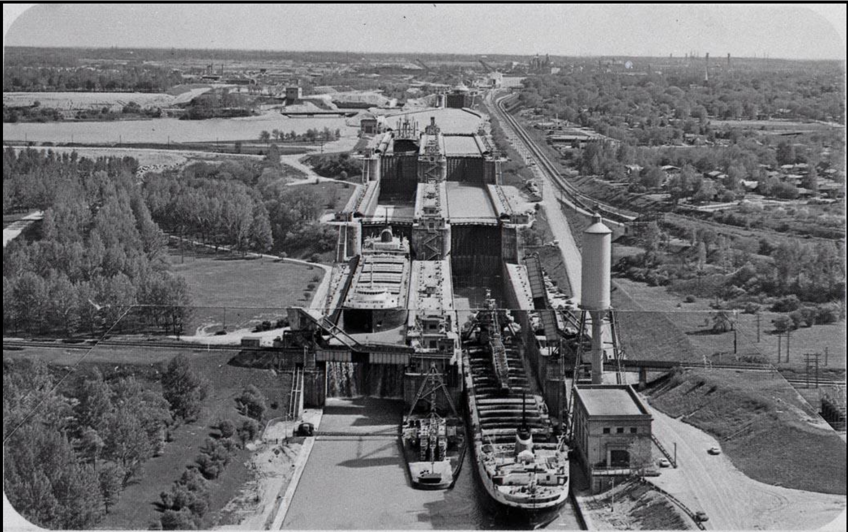
Locks 4, 5, 6 and 7 at Thorold
